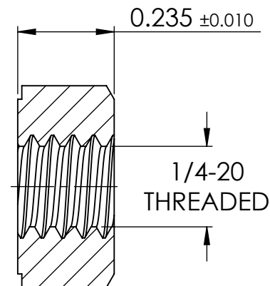
SECTION Y-Y
