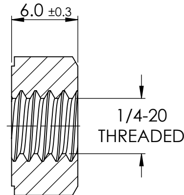
SECTION Y-Y
